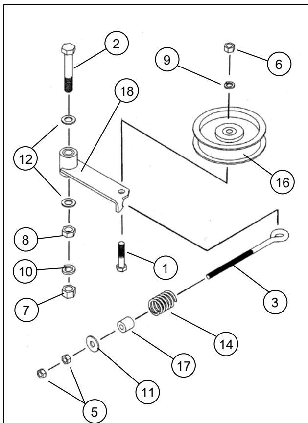
MR55KE Models with a 1.50" Long Spring (Used on Models Built During 2005 & 2006)
