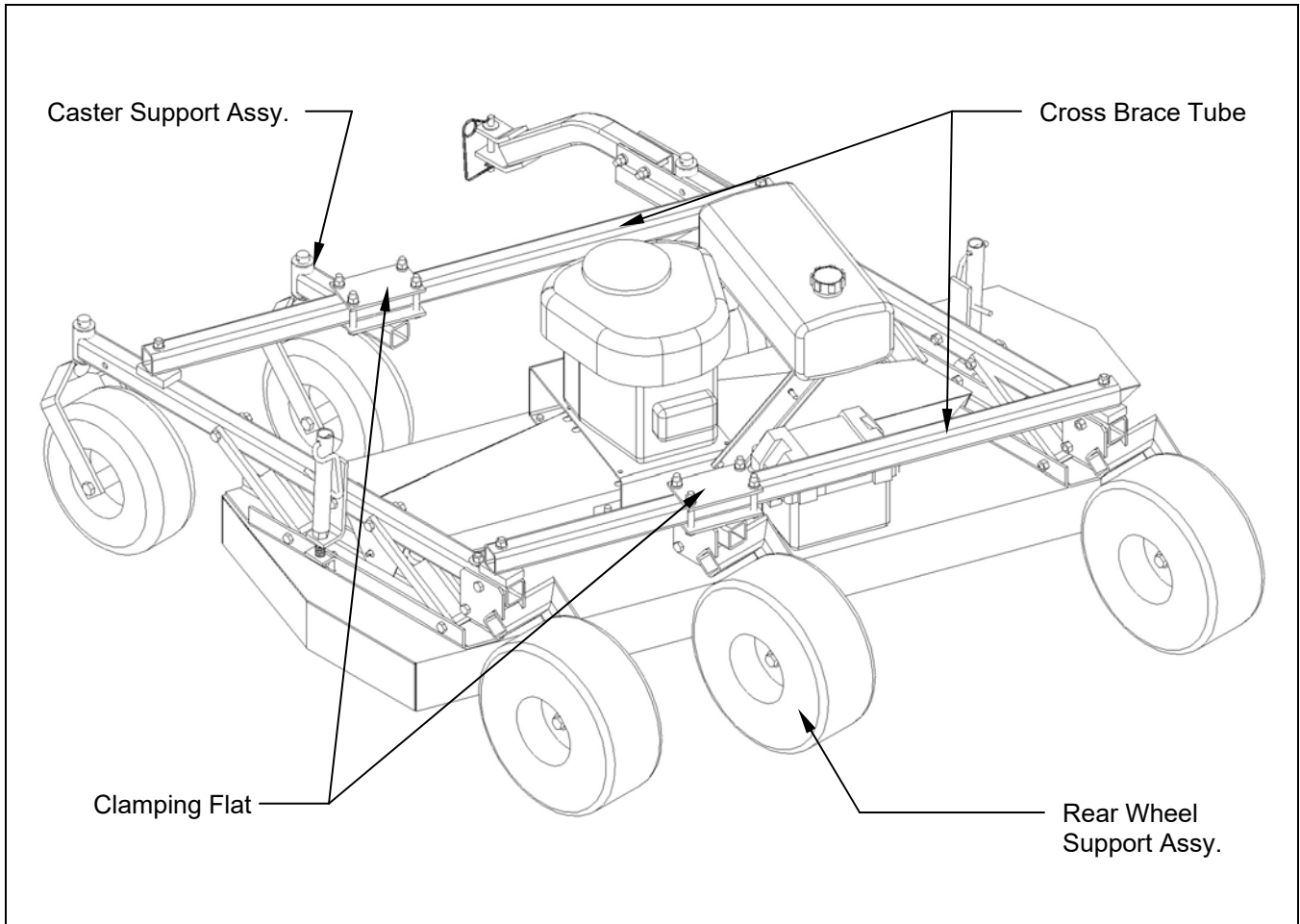
Figure 1: Installation of Floatation Kit Parts
