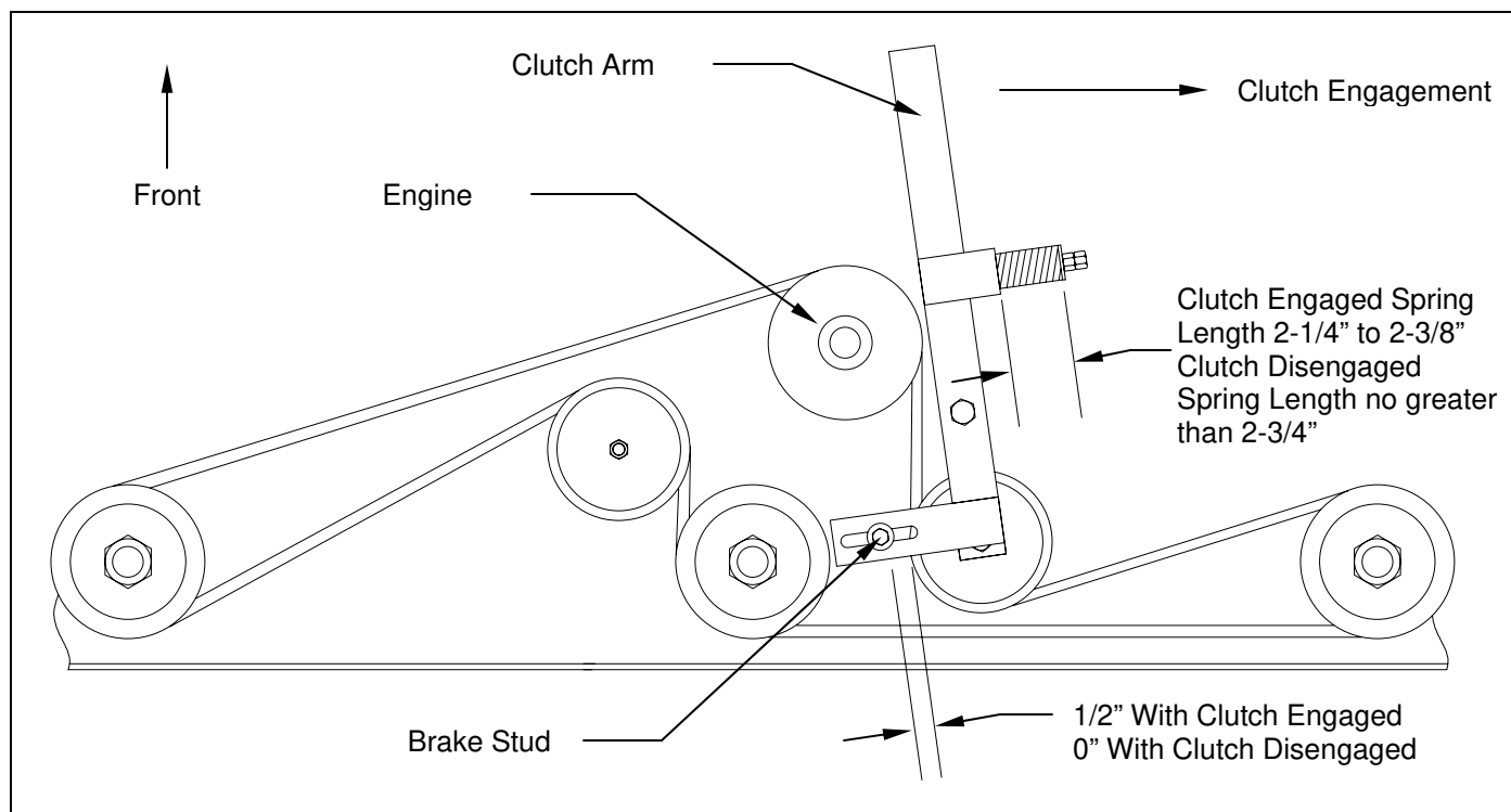
Figure 10: Belt Pattern and Spring Adjustment (Model E60B)
