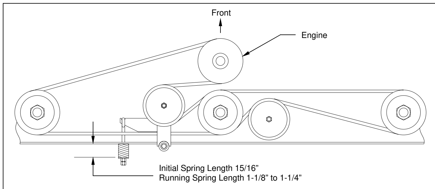
Figure 9: Belt Pattern and Spring Adjustment (Model C60K)
