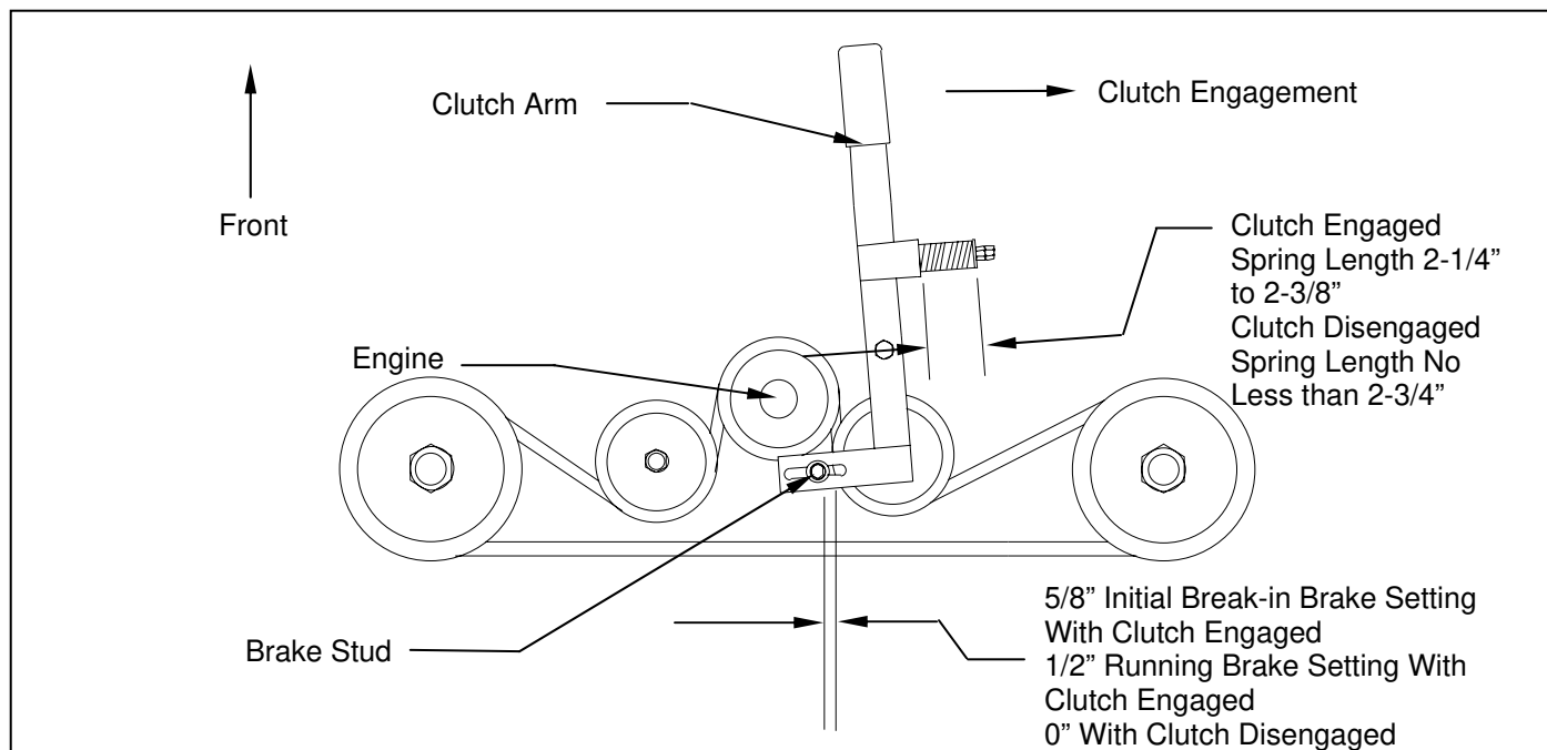
Figure 7: Belt Pattern, Spring Adjustment, and Brake Adjustment
