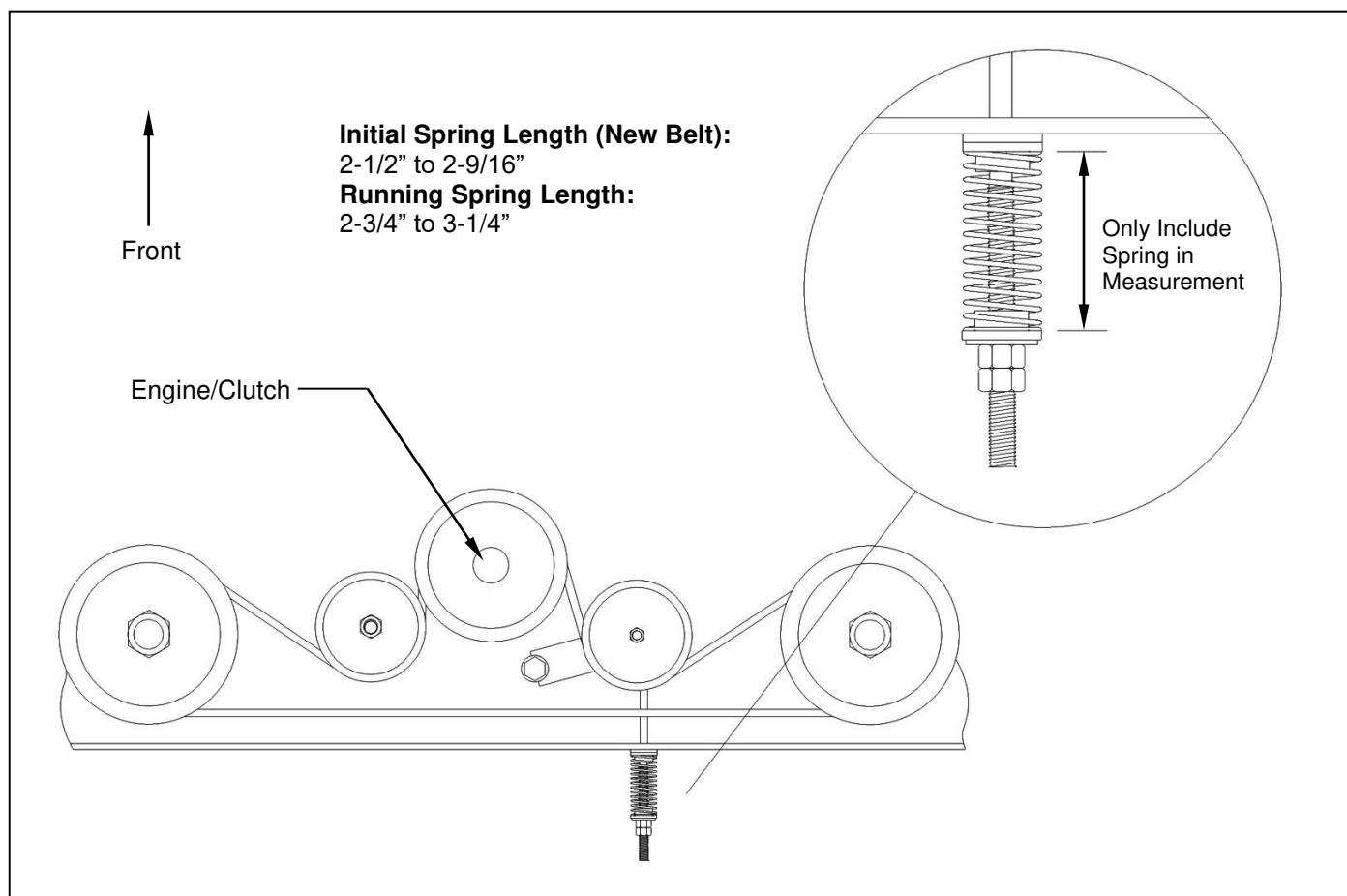
Figure 7: Belt Pattern and Spring Adjustment
